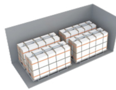
20GP LOADING 2400x1200mm 95"x48"
